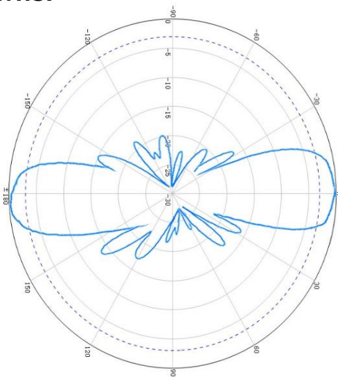
Vertical Pattern – E plane
