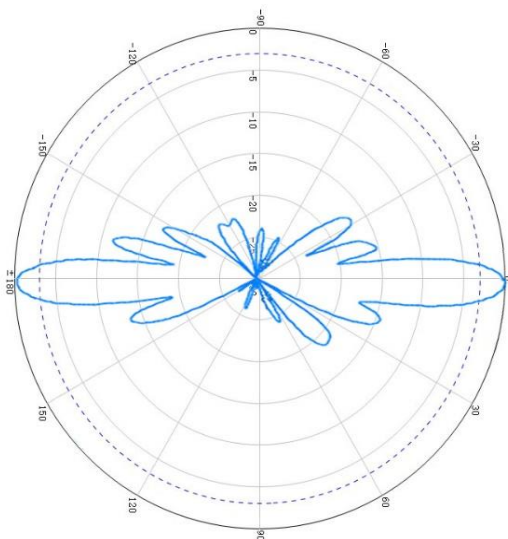
Vertical Pattern – E plane
